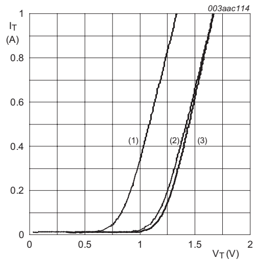
V_o = 0.835 \text{ V}; R_s = 0.50 \Omega (1) T_j = 125^{\circ}\text{C} ; typical values (2) T_j = 125^{\circ}\text{C} ; maximum values (3) T_j = 25^{\circ}\text{C} ; maximum values Fig. 12. On-state current as a function of on-state voltage
