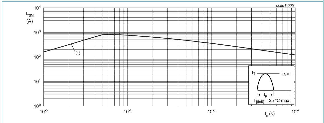
Fig. 5. Non-repetitive peak on-state current as a function of pulse duration; maximum values
