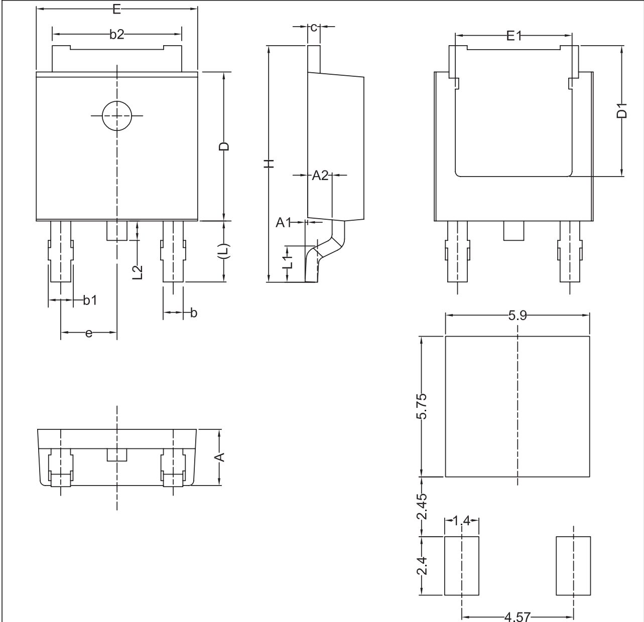
Recommended Footprint
