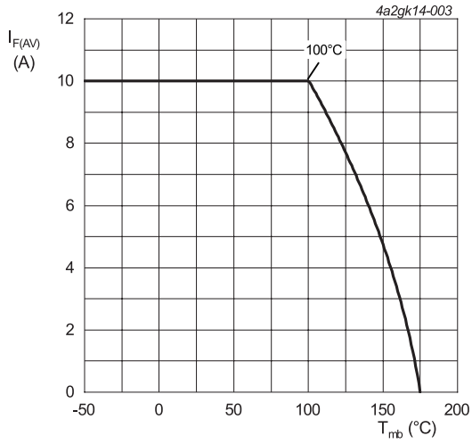
Fig. 3. Forward current as a function of mounting base temperature
