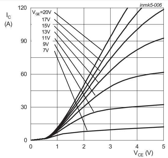
T_j = 175 °C Fig. 6. Typical output characteristic
