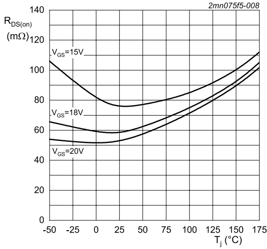
I_{DS} = 20 \text{ A}; t_p < 200 \mu\text{s} Fig. 8. Drain-source on-state resistance as a function of junction temperature
