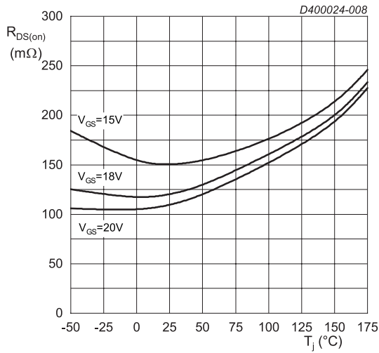
I_{DS} = 10 \text{ A}; t_p < 200 \mu\text{s} Fig. 8. Drain-source on-state resistance as a function of junction temperature
