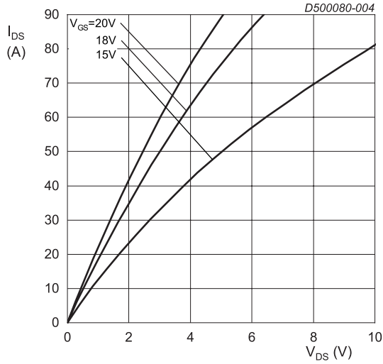
Fig. 4. Output characteristics; drain current as a function of drain-source voltage; typical values T_j = -40\text{ }^\circ\text{C}; t_p < 200\text{ }\mu\text{s}
