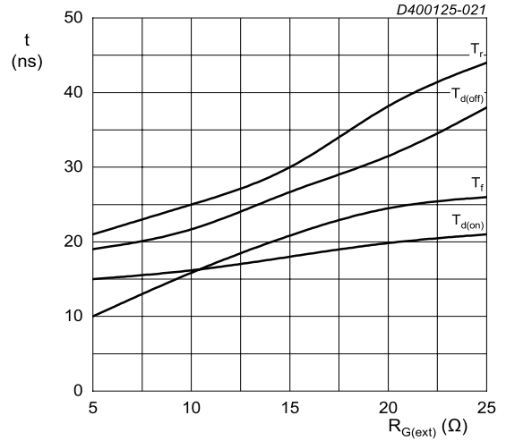
Fig. 21. Switching time as a function of external gate resistance
