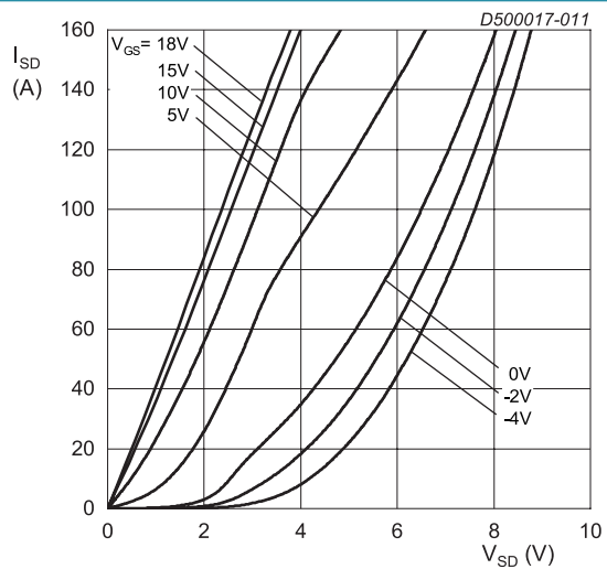
T_j = 25 \text{ }^{\circ} C; t_p < 200 \mu s Fig. 11. Body diode forward characteristics; typical values
