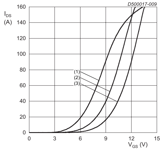
V_{DS} = 20 V; t_p < 200 \mu s (1) T_j = 175 \text{ }^{\circ} C (2) T_j = 25 \text{ }^{\circ} C (3) T_j = -55 \text{ }^{\circ} C Fig. 9. Transfer characteristics; drain current as a function of gate-source voltage; typical values
