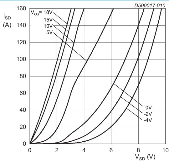
T_j = -55 \text{ }^{\circ} C; t_p < 200 \mu s Fig. 10. Body diode forward characteristics; typical values
