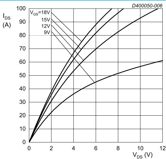
Fig. 6. Output characteristics; drain current as a function of drain-source voltage; typical values T_j = 175\text{ °C}; t_p < 200\ \mu\text{s}
