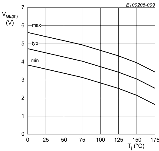
Fig. 9. Gate-emitter threshold voltage as a function of junction temperature
