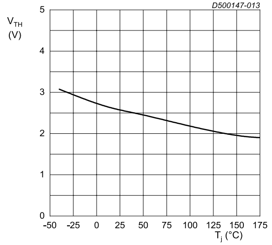
V_{DS} = V_{GS} ; I_{DS} = 24\text{ mA} Fig. 13. Threshold voltage as a function of junction temperature
