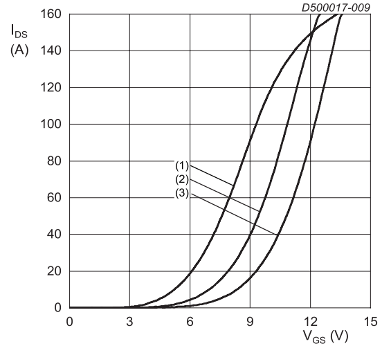
V_{DS} = 20 V; t_p < 200 \mu s (1) T_j = 175 ^{\circ}C (2) T_j = 25 ^{\circ}C (3) T_j = -55 ^{\circ}C Fig. 9. Transfer characteristics; drain current as a function of gate-source voltage; typical values
