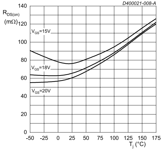
I_{DS} = 20 A; t_p < 200 \mu s Fig. 8. Drain-source on-state resistance as a function of junction temperature
