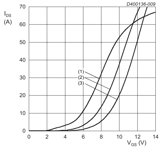
V_{DS} = 20\text{ V}; t_p < 200\ \mu s (1) T_j = 175\ ^{\circ}C (2) T_j = 25\ ^{\circ}C (3) T_j = -55\ ^{\circ}C Fig. 9. Transfer characteristics; drain current as a function of gate-source voltage; typical values
