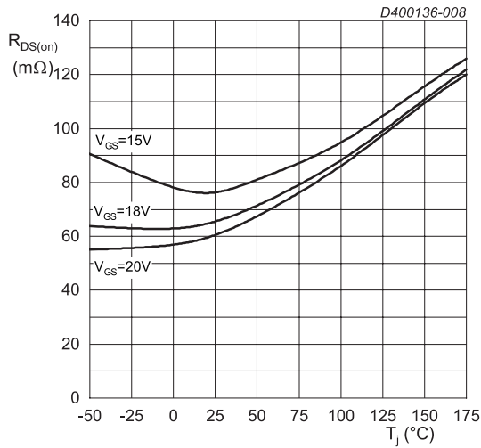
I_{DS} = 20\text{ A}; t_p < 200\ \mu s Fig. 8. Drain-source on-state resistance as a function of junction temperature
